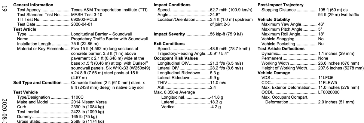
MASH TL-3 CRASH TEST 3-11 (PICK-UP TRUCK) SUMMARY
