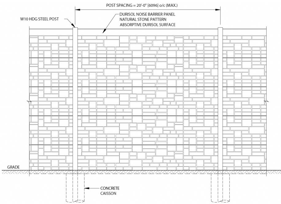
NB20 Simplified Technical Drawing
