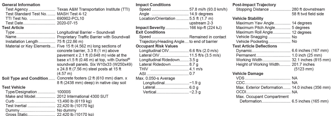
Figure 5.6. Summary of Results for MASH Test 4-12 on Proprietary Traffic Barrier with Inertial Panel and Soundwall System
